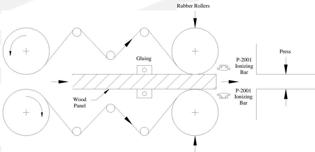
Figure 1: Ionizing bars used in laminating of wood products to neutralize static charges.
